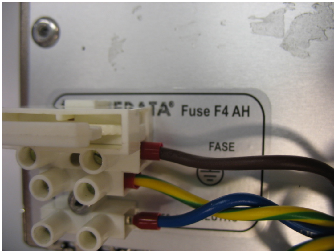
mains terminal with fuse holder
