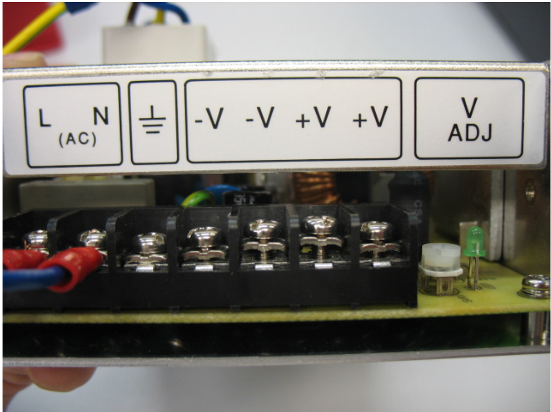
terminal on power supply
